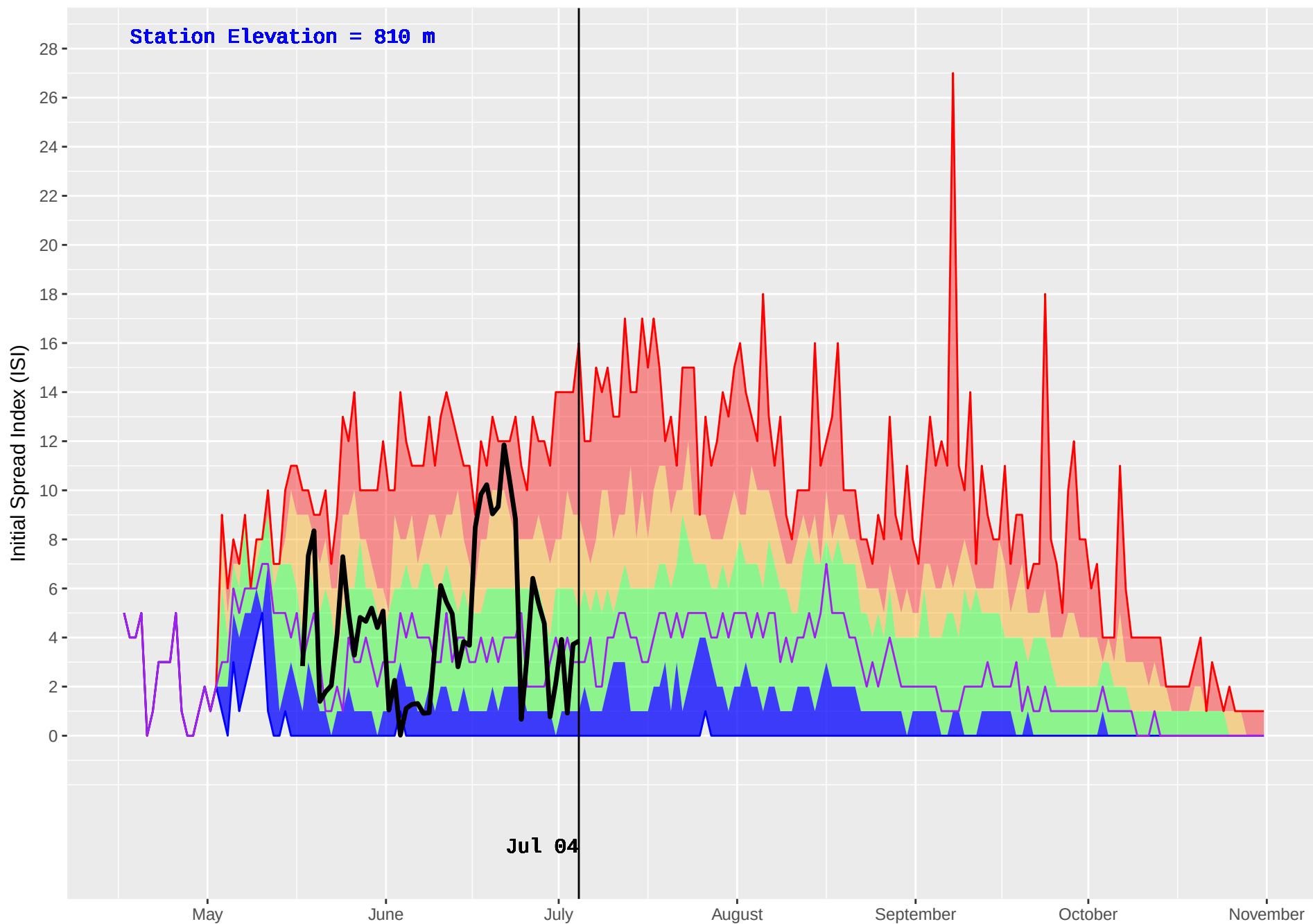
MCBRIDE LAKE (180) : Historical (1990–2016) and Current (2018) Noon Initial Spread Index (ISI)
