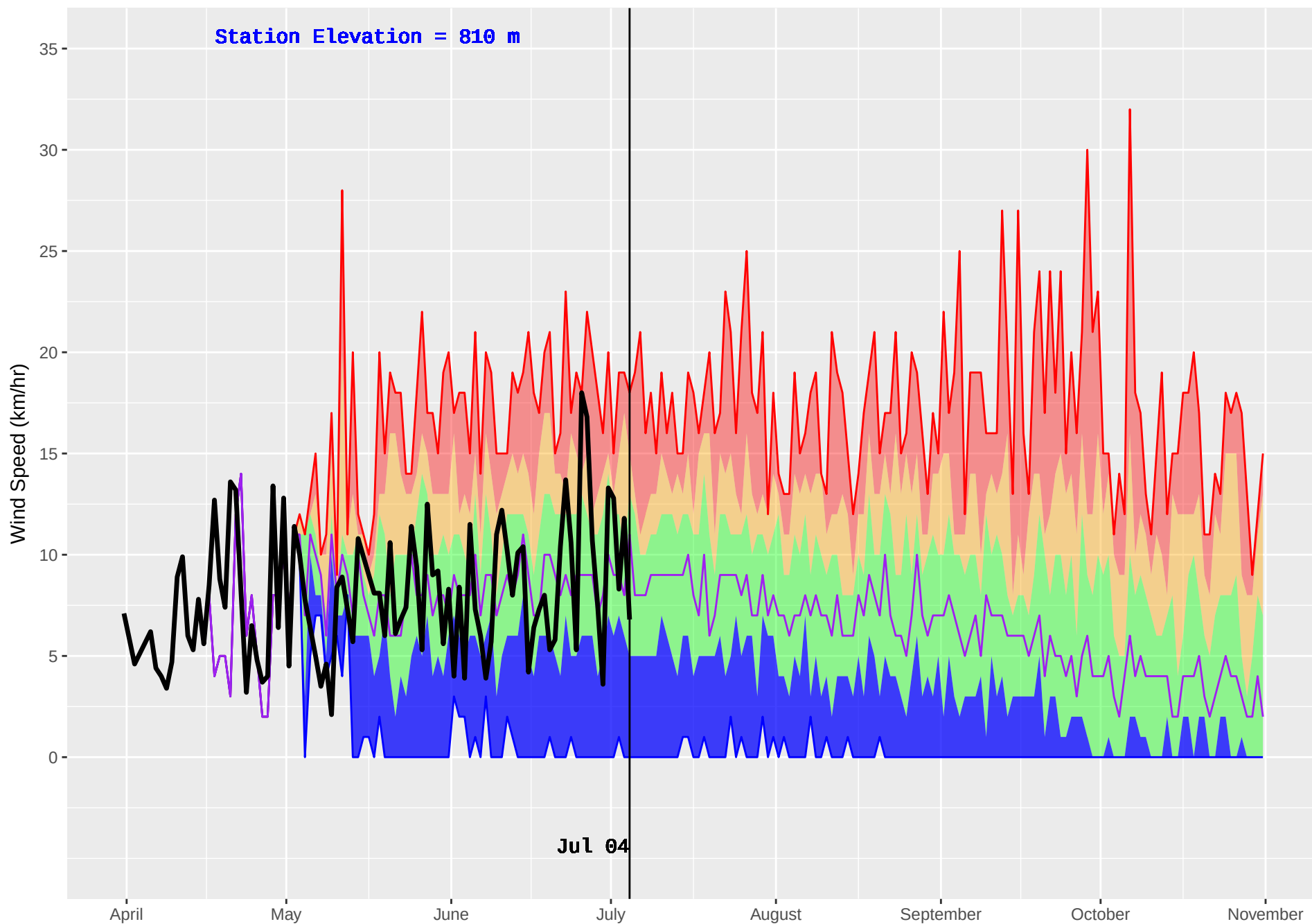
MCBRIDE LAKE (180) : Historical (1990–2016) and Current (2018) Noon Wind Speed
